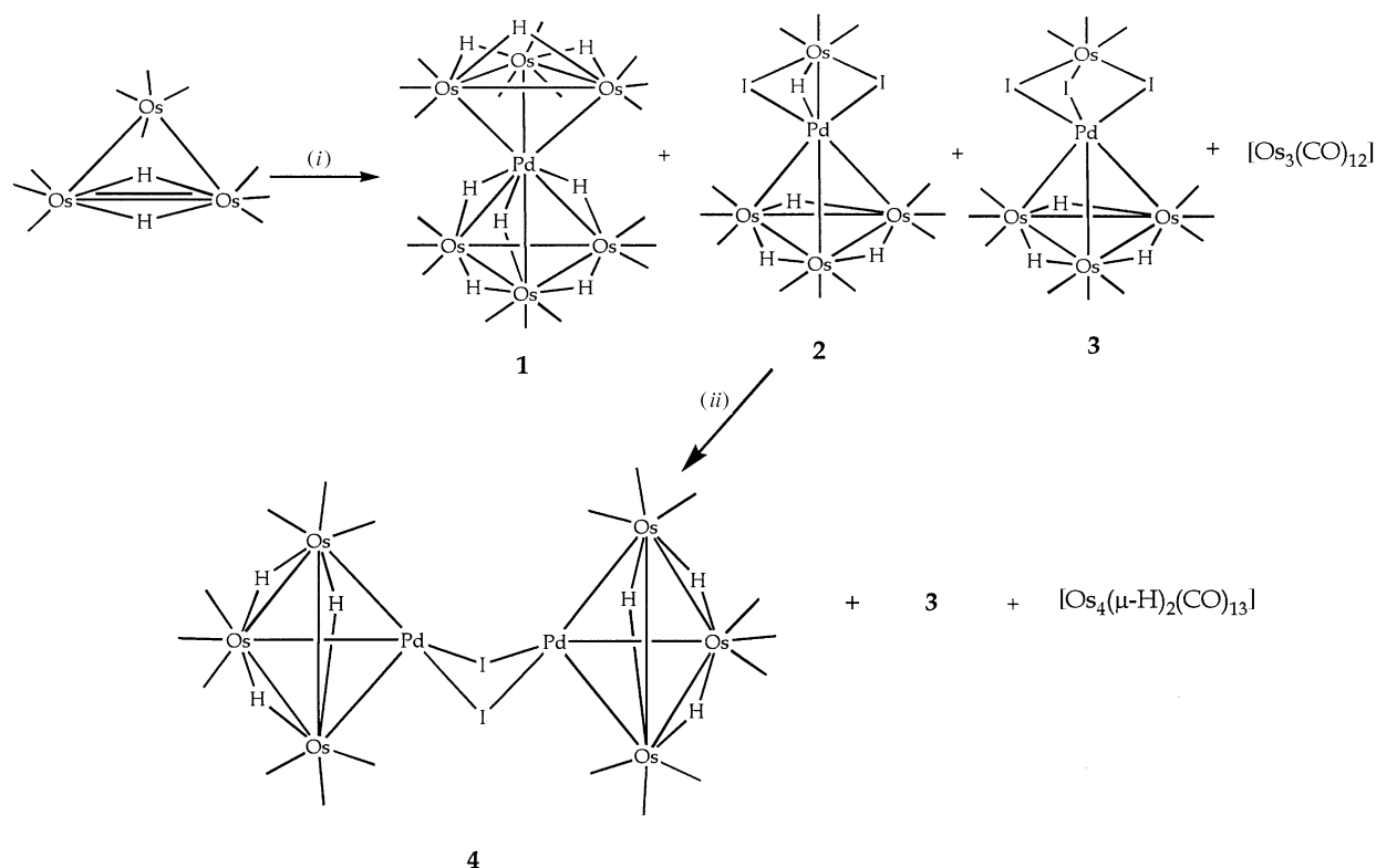
Scheme 1 (i) \text{trans-[Pd(NH}_3)_2\text{I}_2] , room temperature, 4 h; (ii) reflux, \text{CHCl}_3
