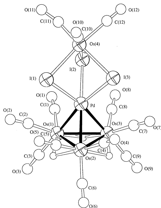
Fig. 3 Molecular structure of complex [Os 4 Pd(μ-H) 3 (CO) 12 (μ-I) 3 ] 3 with the atom numbering scheme
