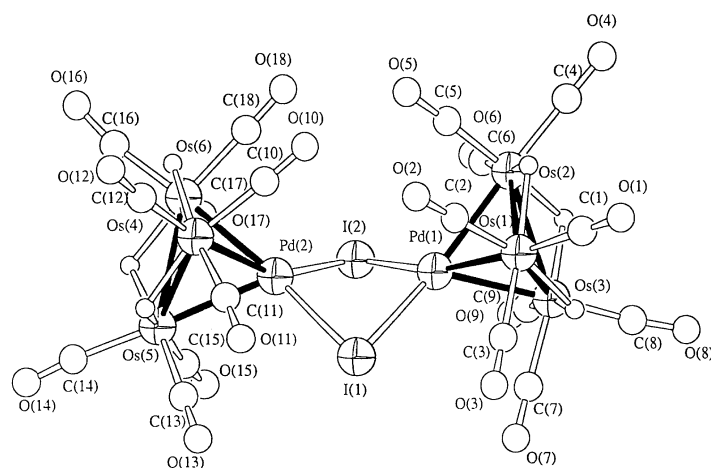
Fig. 4 Molecular structure of complex \{[\text{Os}_3\text{Pd}(\mu\text{-H})_3(\text{CO})_9(\mu\text{-I})_2]\} 4 with the atom numbering scheme
